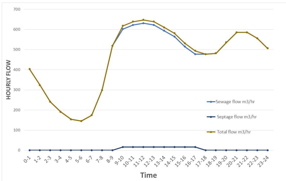
Fig 6: Hourly flow pattern with co-treatment
