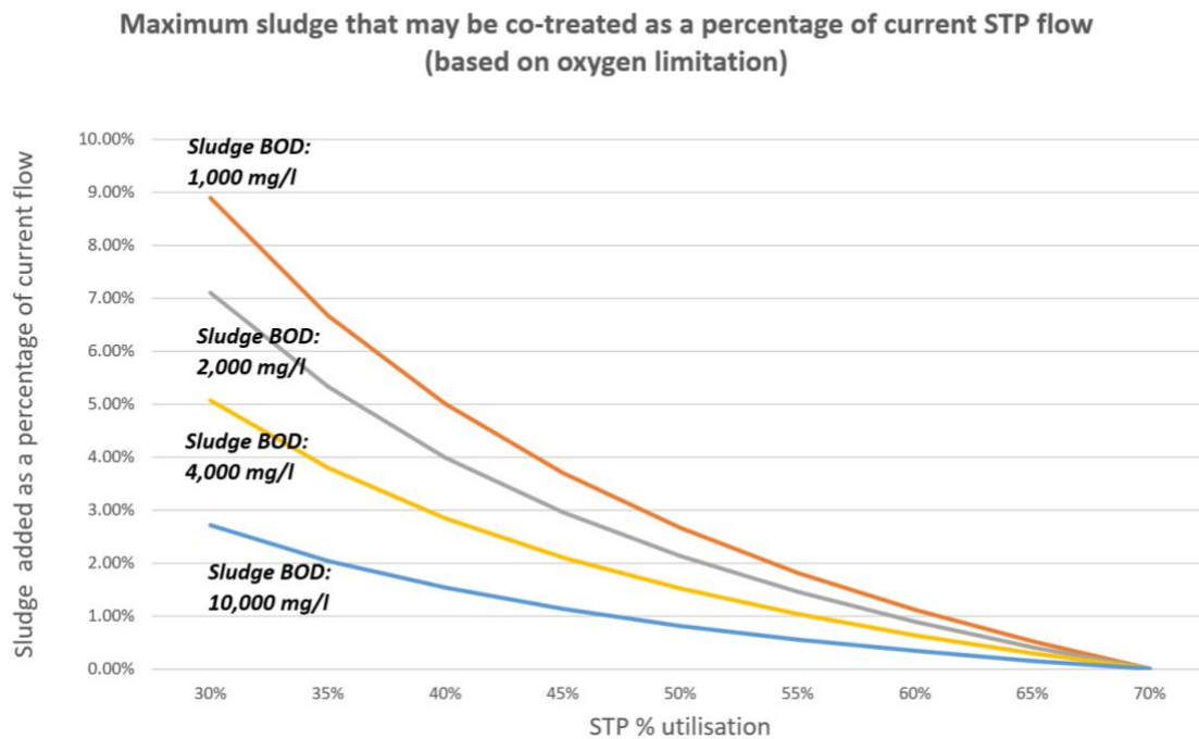
Fig 10: Maximum co-treatment percentage based on oxygen limitation (constant correction factor of 0.7 used)
