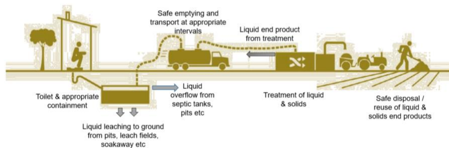
Fig 1: Fecal Sludge Management components
