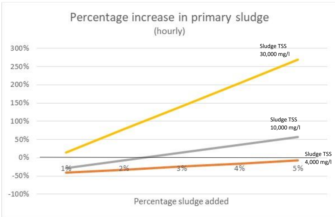
Fig 7: Percentage increase in primary sludge (hourly)
