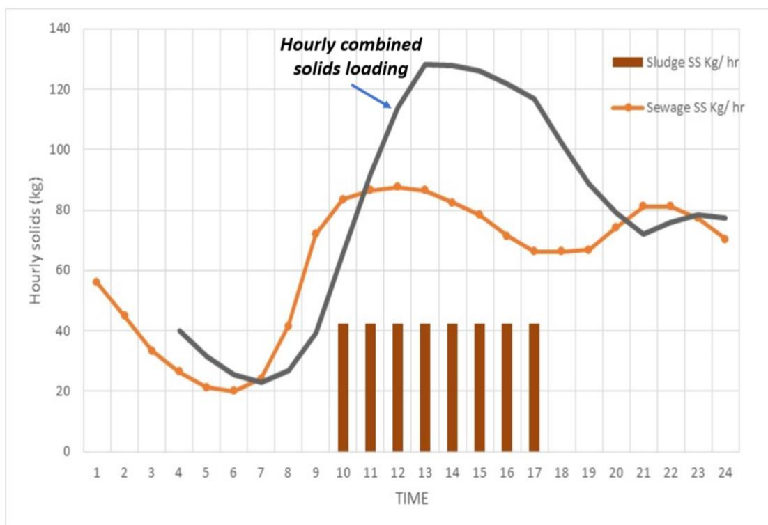
Fig 8: Solids loading under co-treatment conditions.
