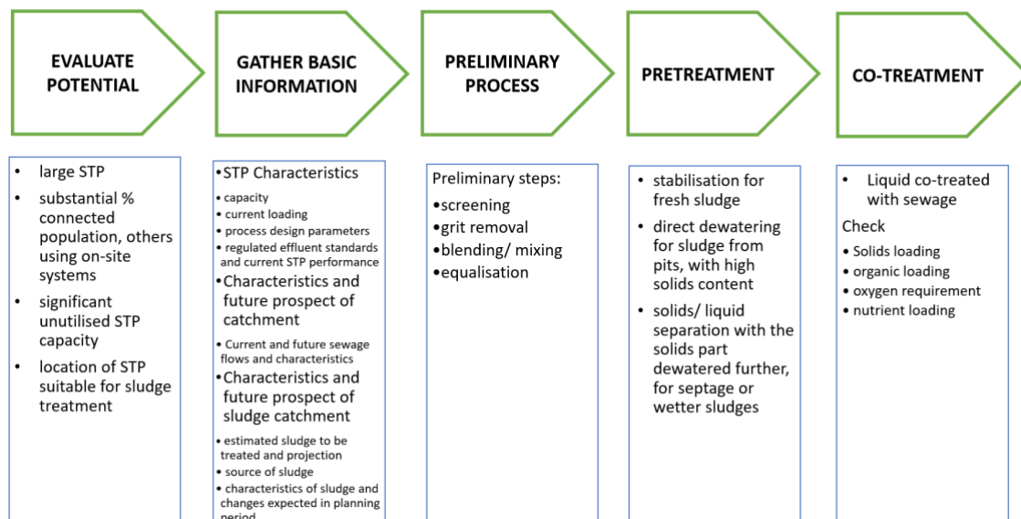
Fig 5: Planning for co-treatment
