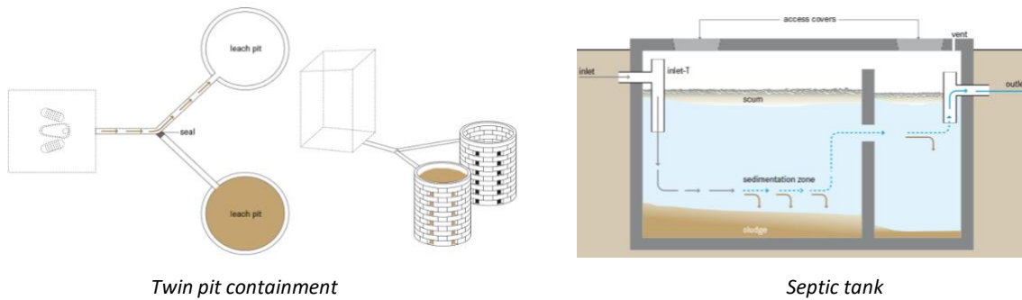
Fig 2: Containment Systems
