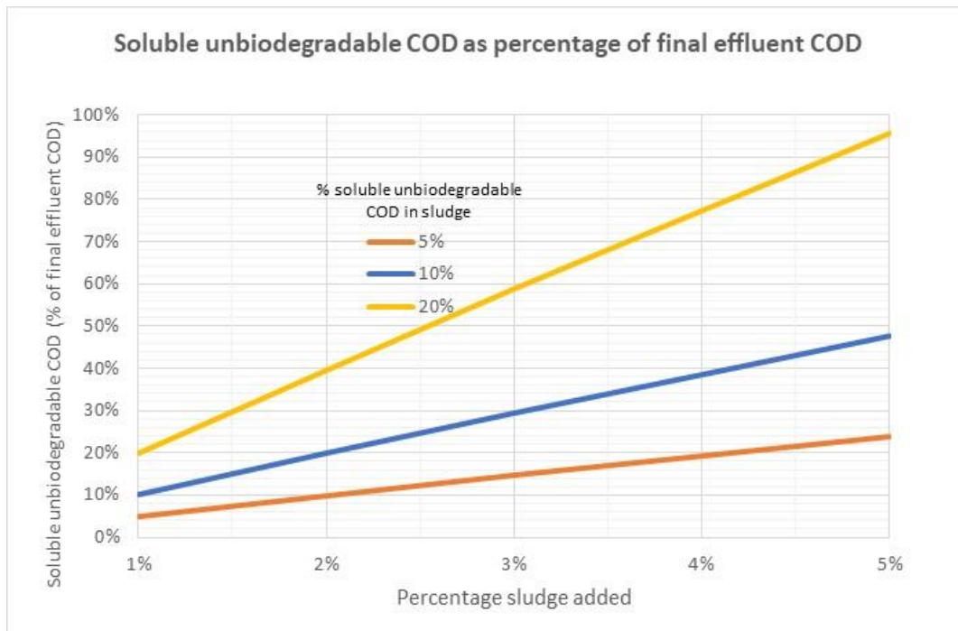
Fig 12: Soluble unbiodegradable COD in final effluent
