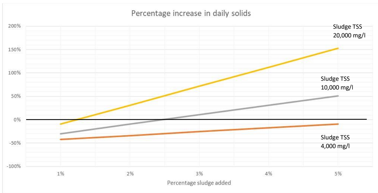
Fig 9: Percentage increase in daily solids loading
