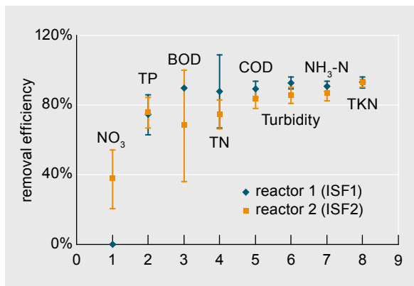
Figure 4: Comparative average removal efficiency in the two reactors with respective feeding frequency of 6/7 and 3/7 days
