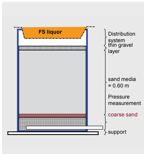
Figure 2: Schematic intermittent sand filters lay out and media sieving
