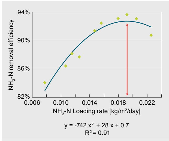
Figure 3: Evaluation of the optimum ammonia nitrogen loading
