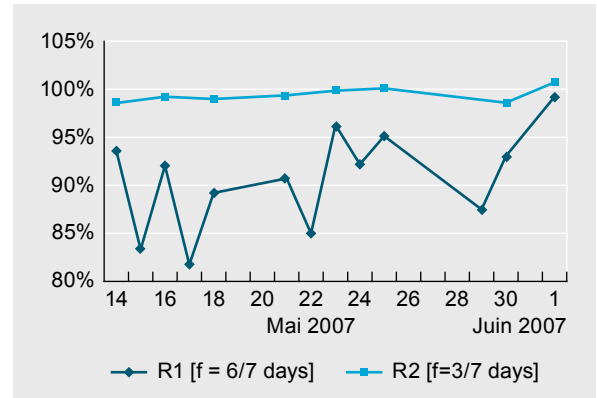
Figure 5: Comparative ammonia nitrogen removal efficiency in the two reactors with respective feeding frequency of 6/7 and 3/7 days
