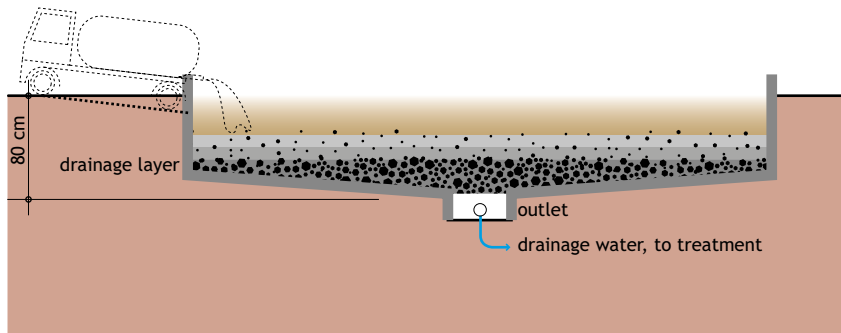
Figure 7.1 Schematic overview of an unplanted sludge drying bed (Tilley et al. , 2014). A splash plate is not visible but is an essential element (Section 7.5).
