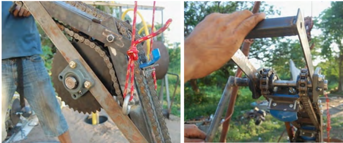
Figure 3.2. First Gobbler prototype
