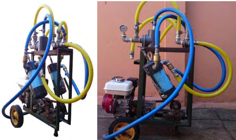
Figure 6.9 Current Nano Vac prototype
