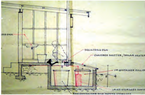
Dehydration toilets with movable bins, Bohol, Philippines
