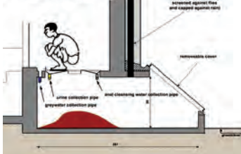
Detail processing Chamber
