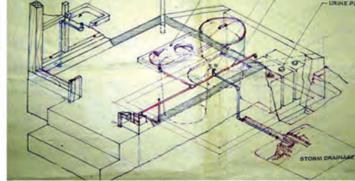
Double-vault dehydration toilets, Bohol, Philippines
