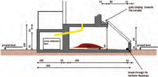
Detail processing Chamber
