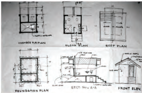
Double-vault dehydration toilets, Bohol, Philippines
