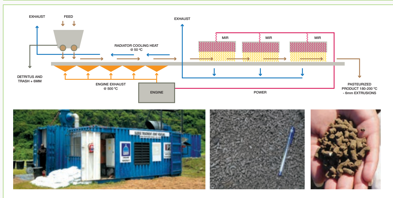
FIGURE 24. LADEPA PILOT PLANT; PELLETS FROM RAW 'SOLID' FS IN SOUTH AFRICA.
