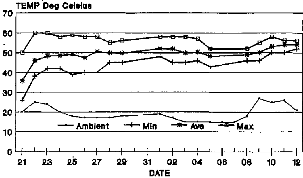
Windrow no.1 : 21 May - 12 June 1992
