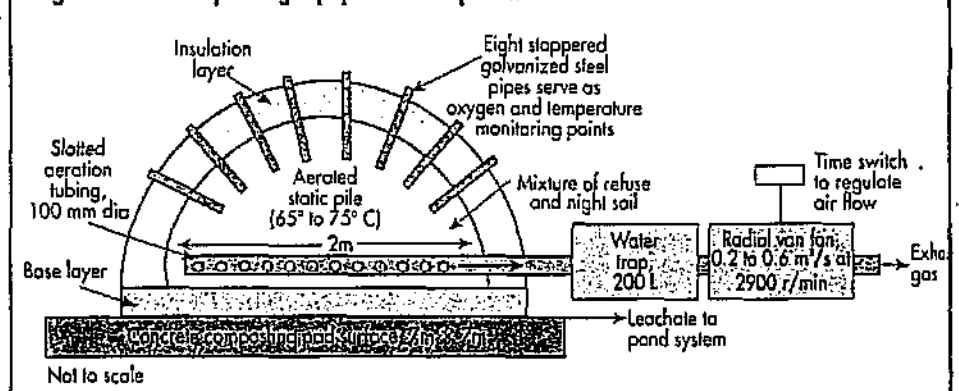
Figure 2—Co-composting Equipment Components
