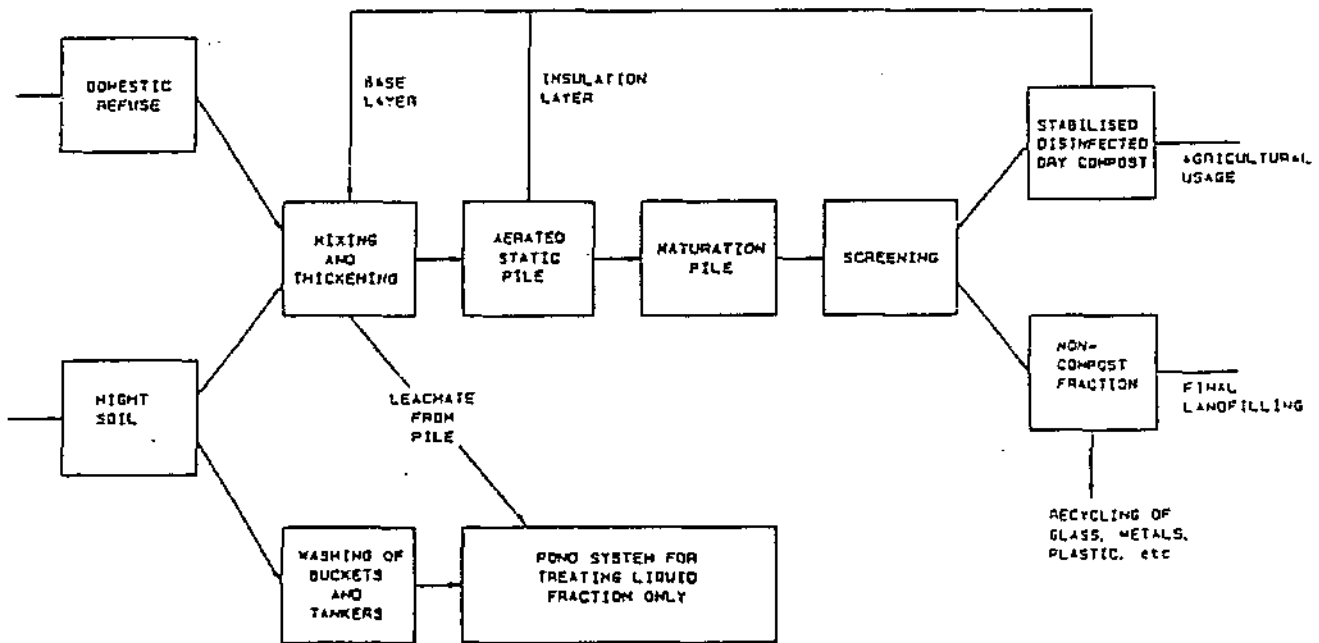
Figure 2: Unit operations of the forced aeration static pile Composting Of Refuse And Night Soil (CORANS) Process.
