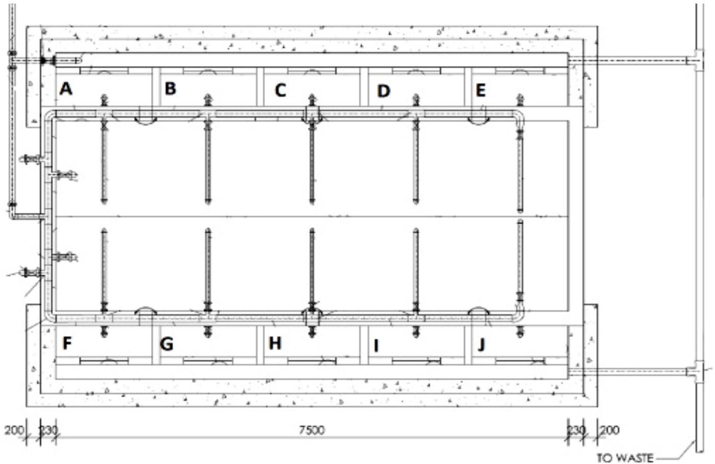
Figure 1. Schematic representation of a multi-designed wetland system in Durban.
