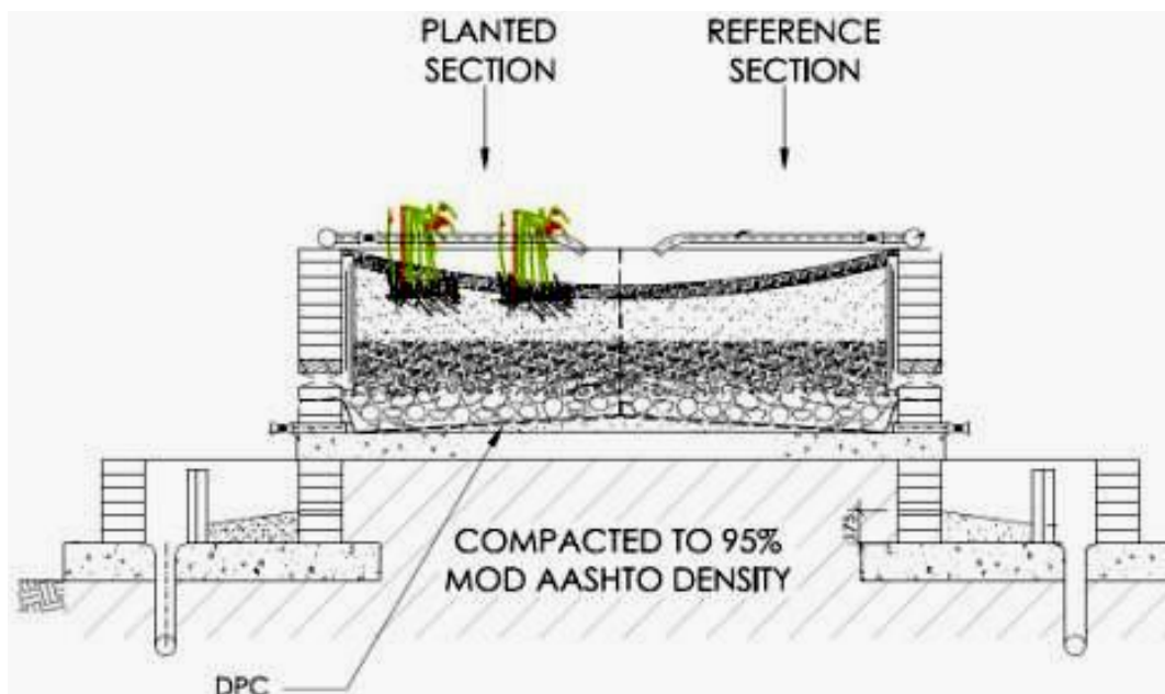
Figure 2. Cross section of the multi-engineered system. The plants are planted in such a way that they are evenly distributed across the test section of the wetland. The layout of plants in the wetland medium can be seen in Figure 1. Species of the plants used are Phragmites australis .
