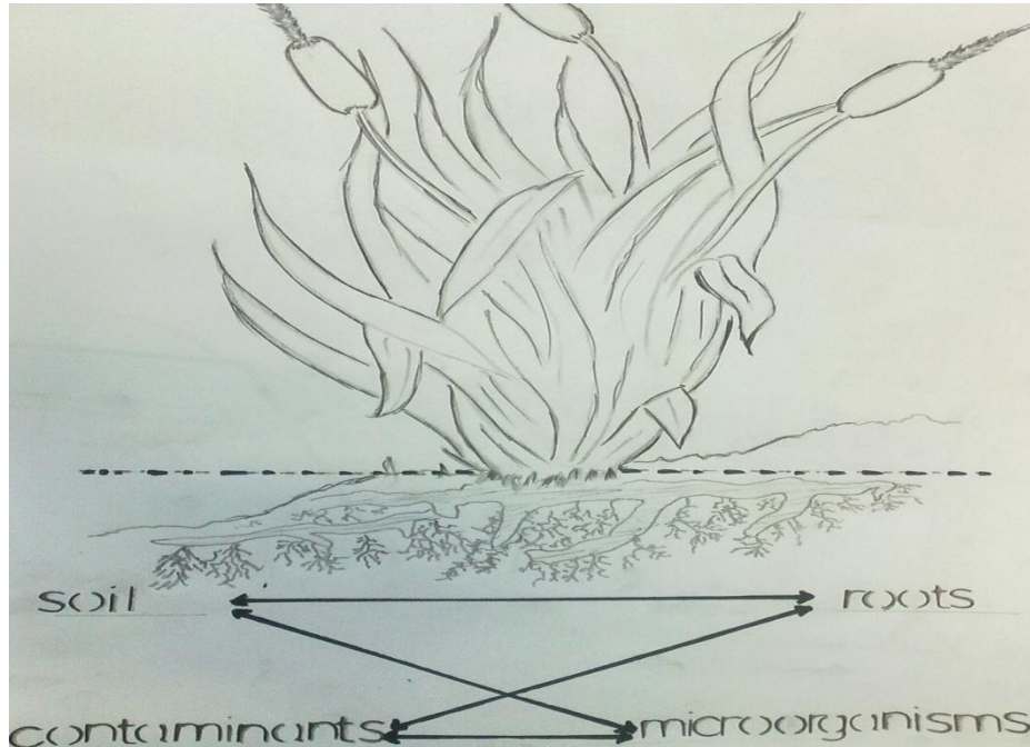
Figure 5. Some possible interactions occurring in wetlands (Stottmeister et al., 2003).
