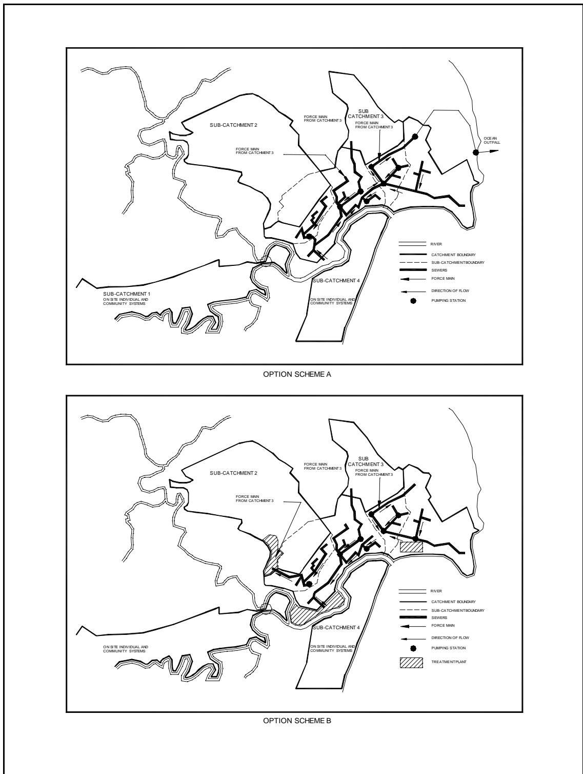
Figure 9.1 Option Scheme A & B
