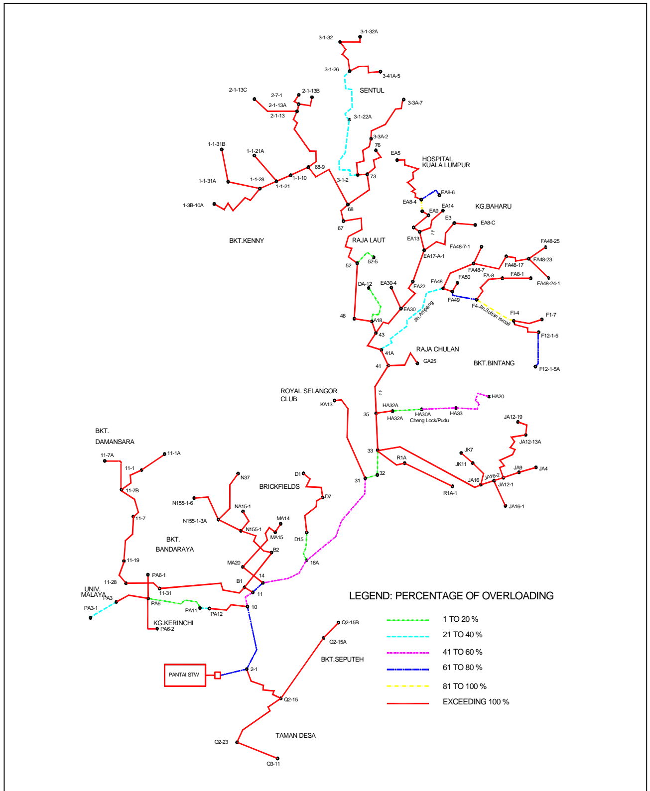
Figure 6.1 Status of Pantai Sewerage Zone Network System (Flow Conditions for Year 2000)
