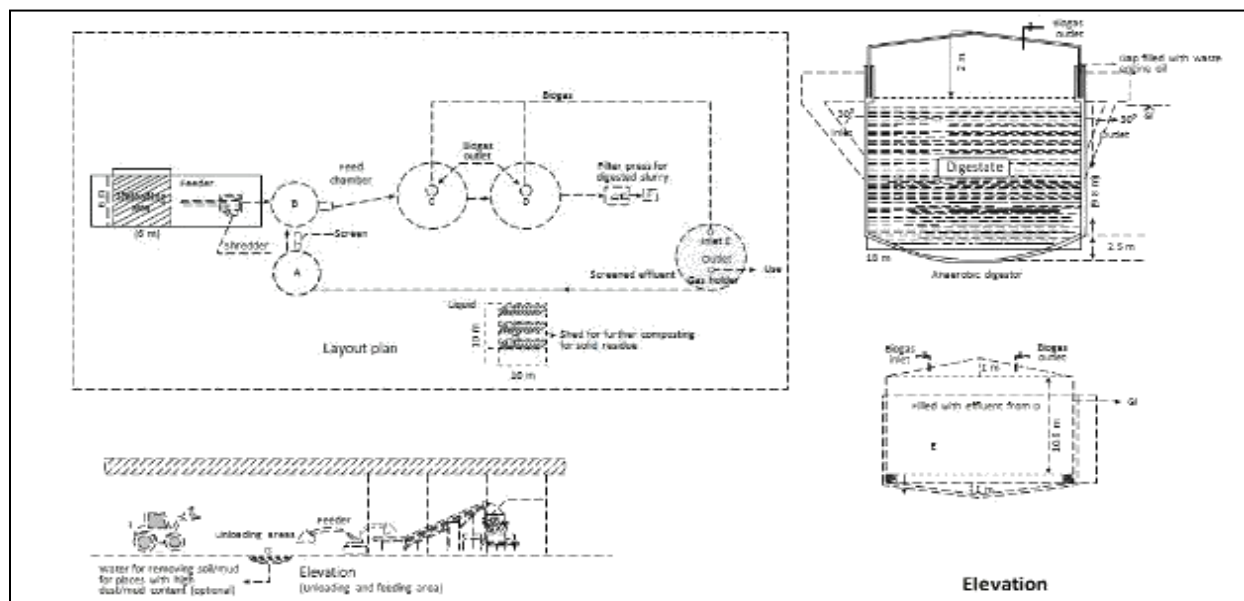
Figure 19: Biomethanation plant for 50 TPD of waste
