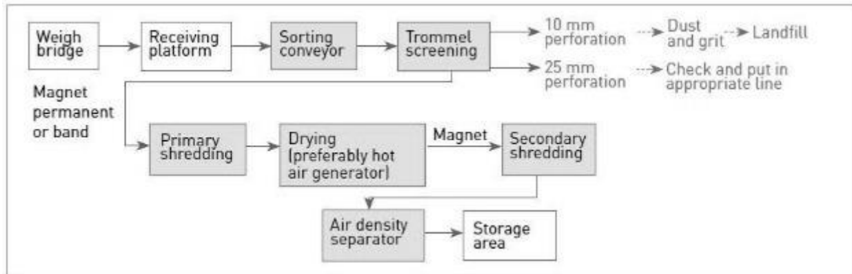
Figure 17: Indicative Material Recovery Facility and Pre-sorting Facility dedicated to Dry waste
