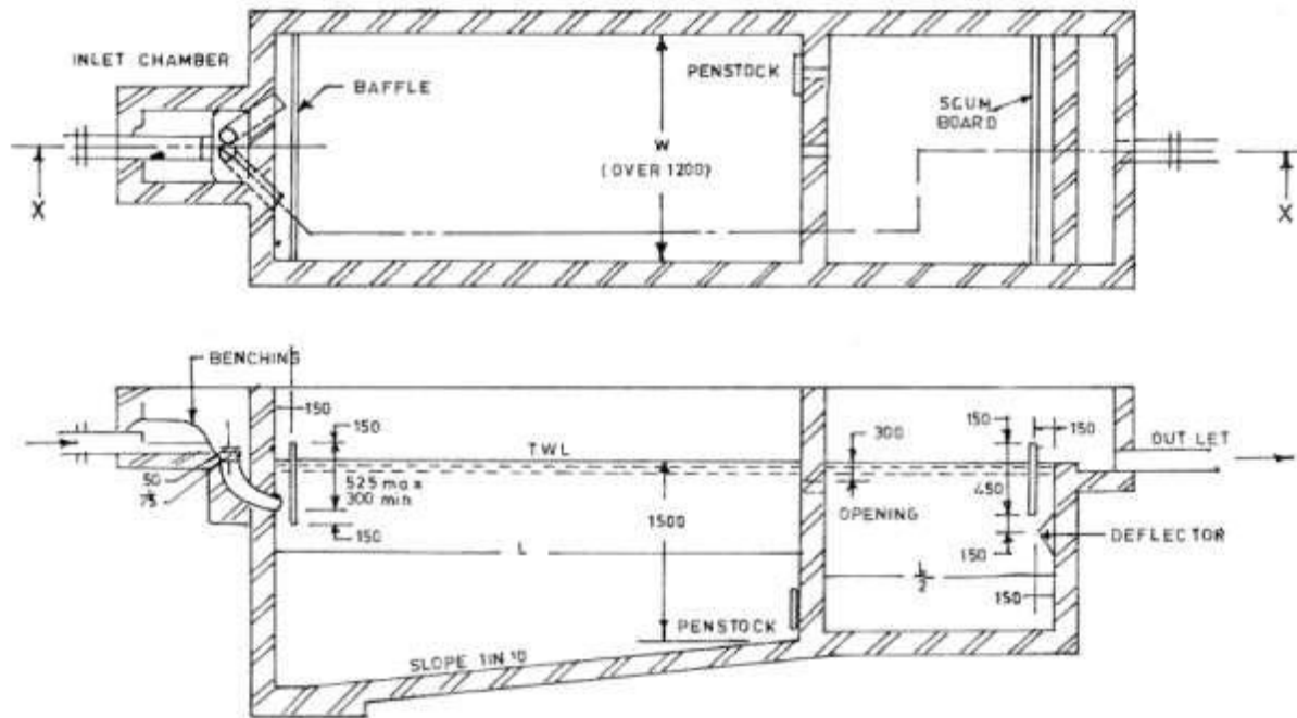
Figure 16: Typical sketch of a two- compartment septic tank for 5 users (dimensions in mm)
