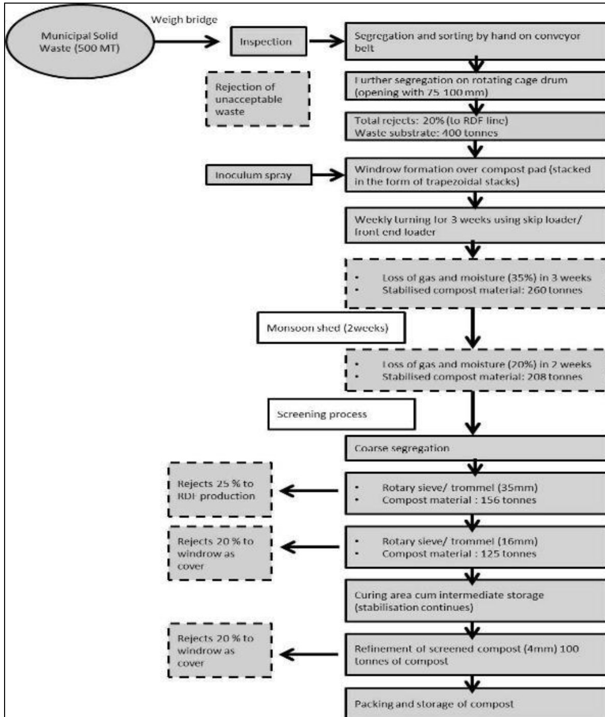
Figure 18: Process Flowchart and mass balance for anaerobic windrow composting of 500 MT per day of waste of waste
