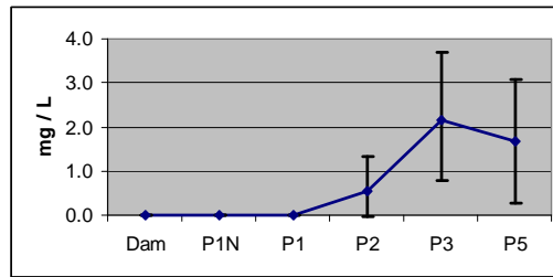
Figure 31: Dissolved oxygen concentration evolution in Network 4
