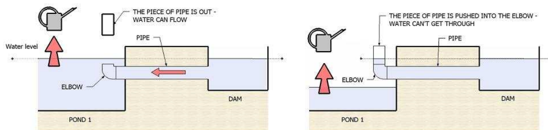
Figure 20: Sketch of floodgate system used in Network 4
