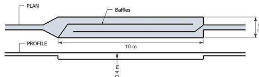
Figure 17: Plug flow retention pond in Network 1
