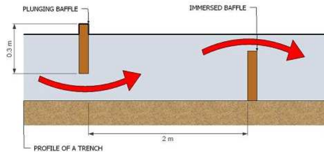
Figure 16: Plunging and immersed baffles
