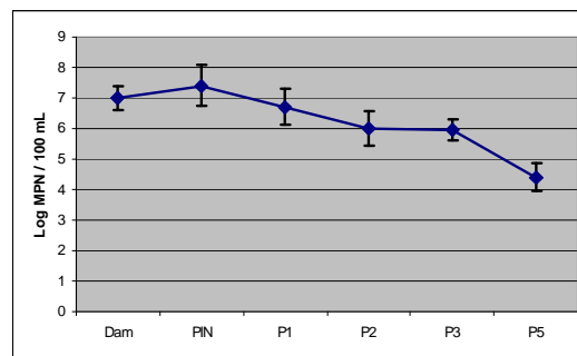
Figure 29: Faecal coliform concentration evolution along Network 4 in May-June
