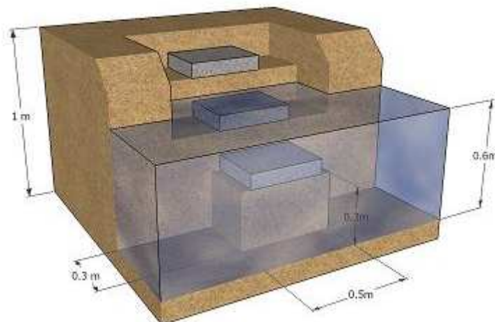
Figure 15: Improved fetching point – first design
