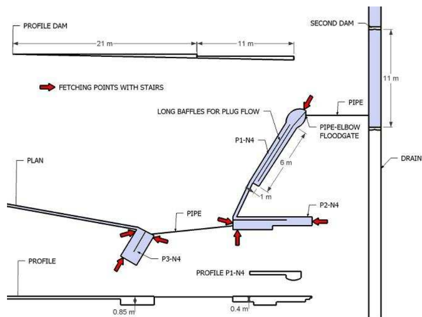
Figure 19: Sketch of the main modifications in Network 4
