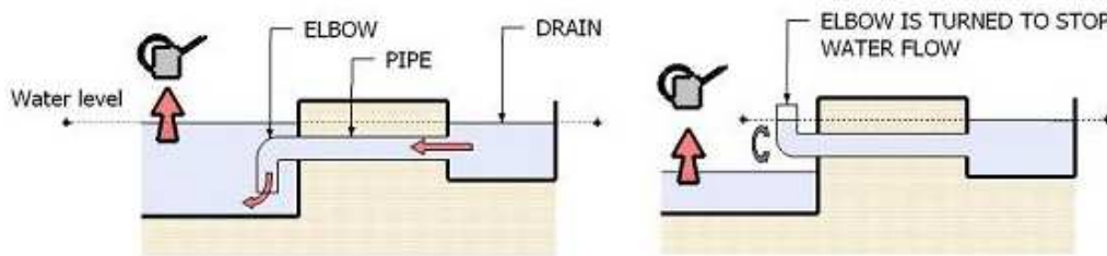
Figure 21: Sketch of the floodgate system with an elbow in the pipe
