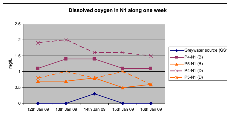
Figure 6: Graph of dissolved oxygen results in Network 1
