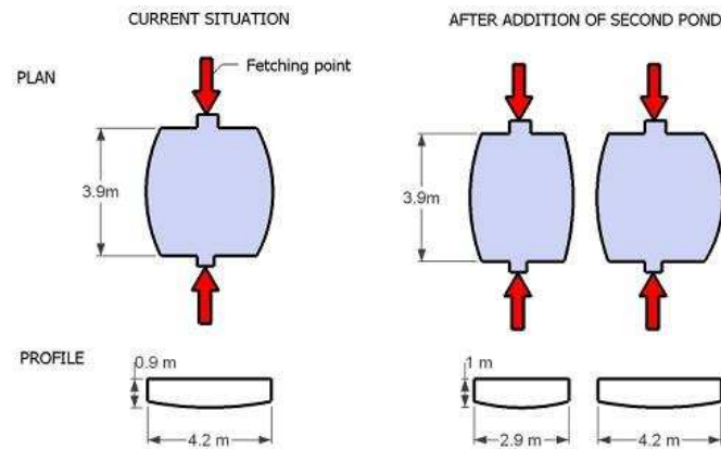
Figure 23: Sketch of modifications planned with Pond Y
