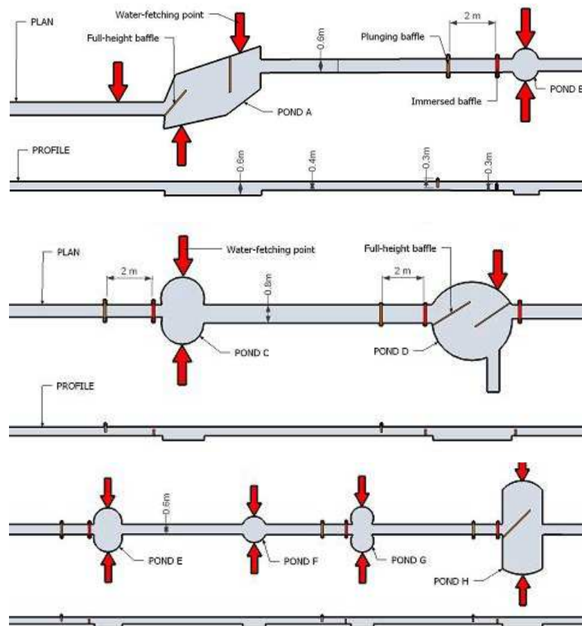
Figure 18: Planned modifications in Network 1
