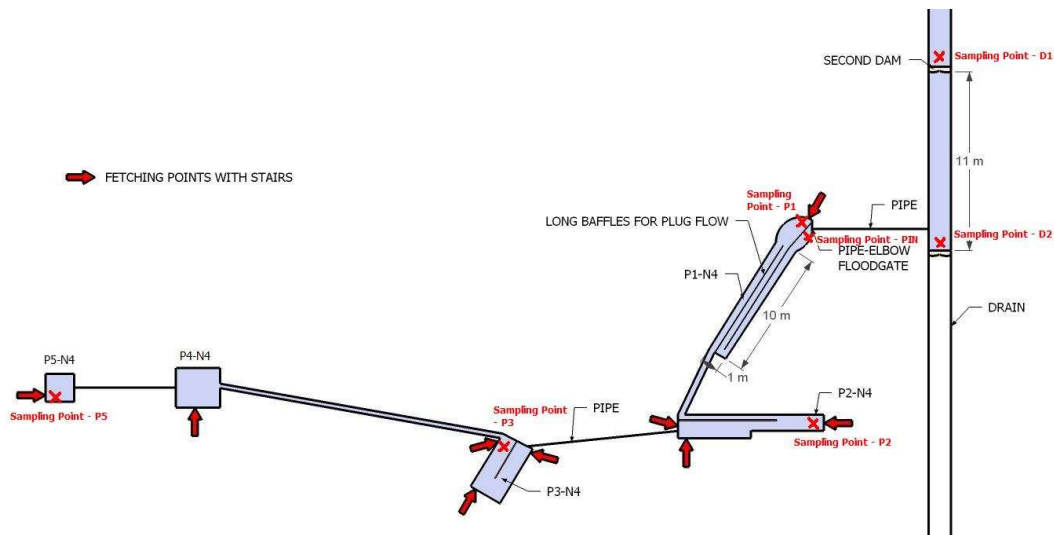
Figure 27: Location of sampling points in Network 4
