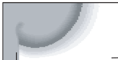
Figure 14: Modeling of a coliform pulse diffusion in a pond with baffles
