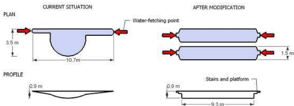
Figure 24: Sketch of modifications planned with Pond H
