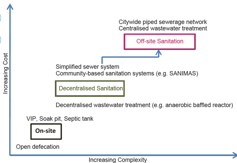
Figure 6. Decentralized sanitation fills the gap between on-site and centralized sanitation options (Source: Modified from (WSP, 2013))
