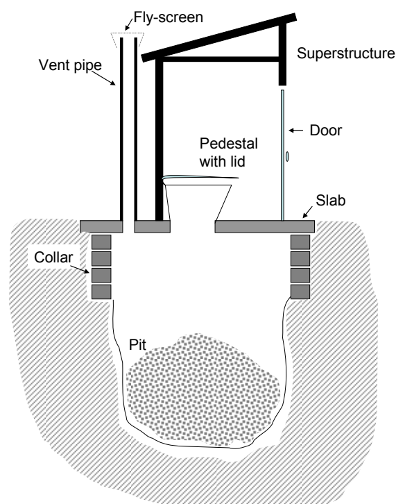
Figure 1: Basic structure of a VIP
