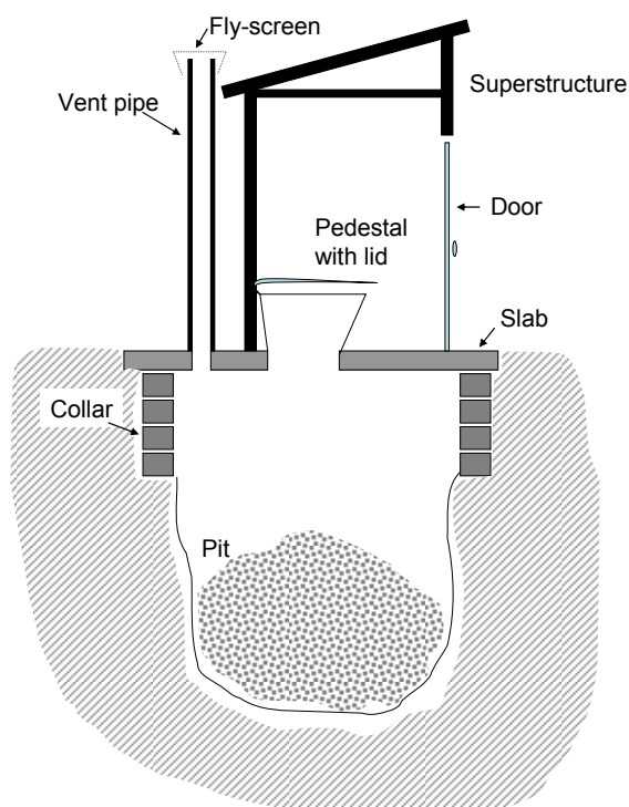
Figure 1.2: Basic structure of a VIP
